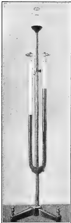
Apparatus for separating water into the two elements hydrogen and oxygen.
