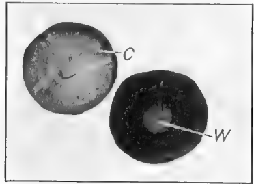
A cross section through a taproot (a parsnip): C, cortex; W, wood. Notice in the right-hand specimen, which has been dipped in iodine, that the core of wood continues out into the rootlets which leave the main root. Where is most starchy food stored in a parsnip?
