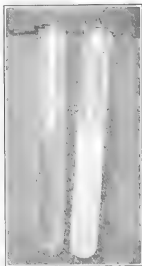
The limewater test; the tube at the right shows the effect of carbon dioxide.
