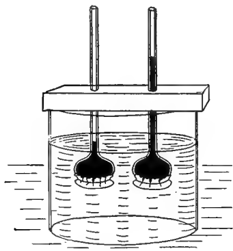
Experiment showing the osmosis of sugar (right-hand tube) and non-osmosis of starch (left-hand tube).
