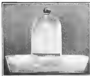
Experiment to show the amount of nitrogen present in the air.
