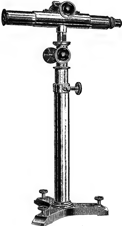
FIG. 98.—Horizontal microscope.
