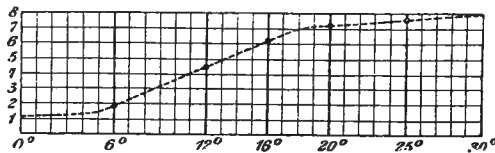
FIG. 71.—Graph representing relation of temperature to velocity of penetration of water through the protoplasmic membrane.
