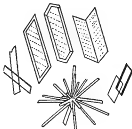
FIG. 52.—Crystals of potassium chloroplatinate. FIG. 53.—Crystals of calcium sulphate.
