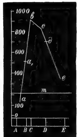
FIG. 13.—Graphs showing relative rates of decomposition of carbon dioxide in different parts of the spectrum. (After Timiriazev.)
