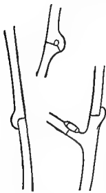
Fig. 62.—Clamp-connections.
