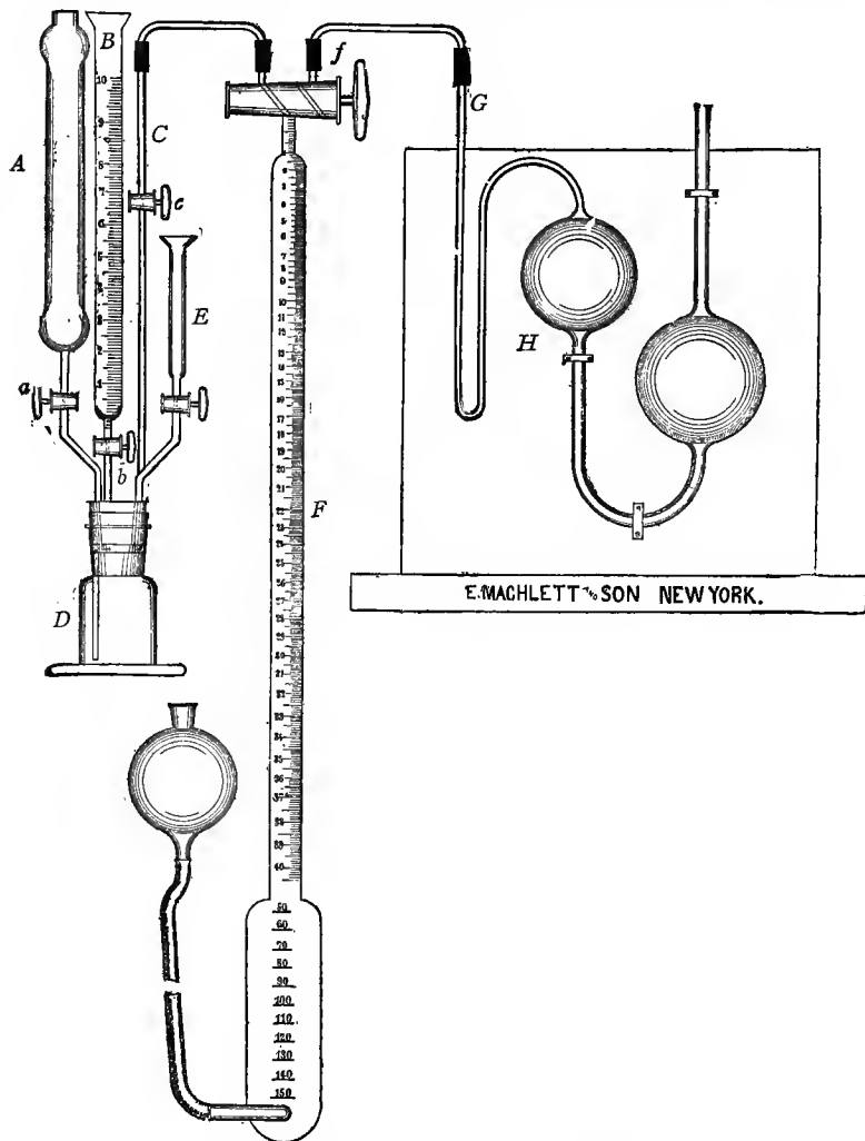
FIG. 12.—Van Slyke's Amino Nitroger Apparatus.
