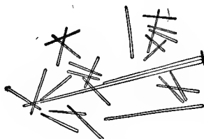
FIG. 3.—Ergotoxine Hydrochloride.
