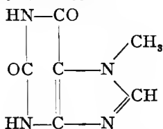
Epiguanine. 7-methyl-2-amino-6-oxypurine.
