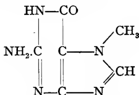
Epiguanine. 7-methyl-2-amino-6-oxypurine.
