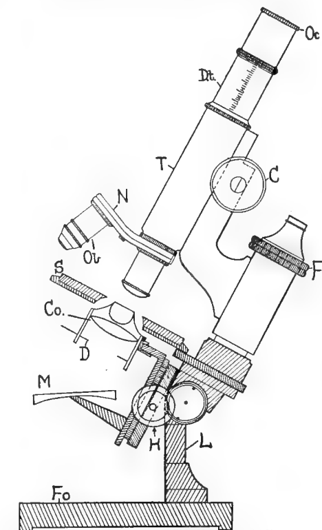
FIG. 230.—Diagrammatic representation of a compound microscope. C. , Coarse adjustment; Co. , condenser; D. , diaphragm; D.t. , draw-tube; F. , fine adjustment; Fo. , foot; H. , milled head controlling substage adjustment for condenser; L. , pillar; M. , mirror; N. , nosepiece; Ob. , objective; Oc. , ocular or eyepiece; S. , stage; T. , body tube.
