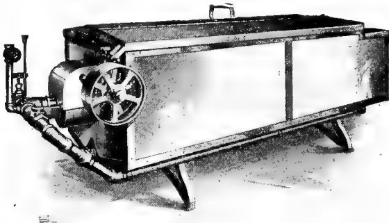
FIG. 72.—Wizard vat pasteurizer and cream-ripener. (Creamery Package Mfg. Co)
