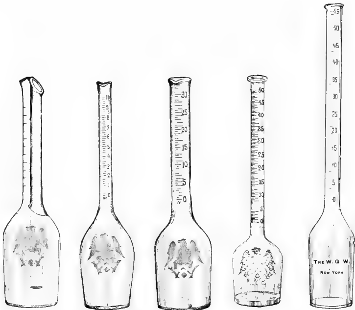
FIG. 22. Skim-milk test-bottle. FIG. 23. Whole-milk test-bottle. FIG. 24. Cream test-bottle. FIG. 25. 9-gram cream test-bottle. FIG. 26. Cream test-bottle. Babcock Test-bottles.
