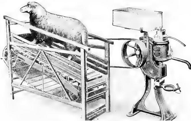
FIG. 57.—Tread-power attached to United States hand separator.
