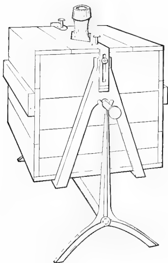
FIG. 20.—Acid carboy trunnion.
