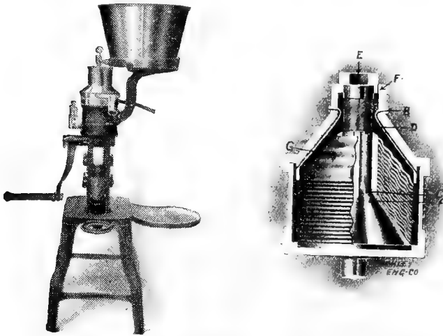
FIG. 55.—Peerless hand separator and cross-section of bowl.
