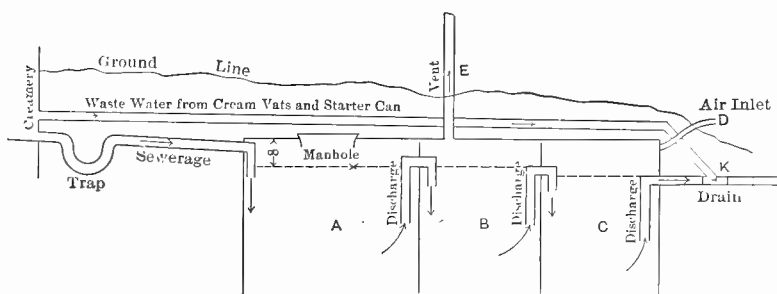
FIG. 123.—Septic tank for creamery sewage disposal. (By Prof. J. Michels.) The tank should be located in the ground with the top within a foot or two of the surface. It may be constructed of planks. Brick, stone, or concrete is preferable for durability. The tank should be built air-tight except in two places, D and E.
