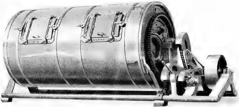
FIG. 88. Disbrow churn (Davis-Watkins Dairymen's Mfg. Co.)
