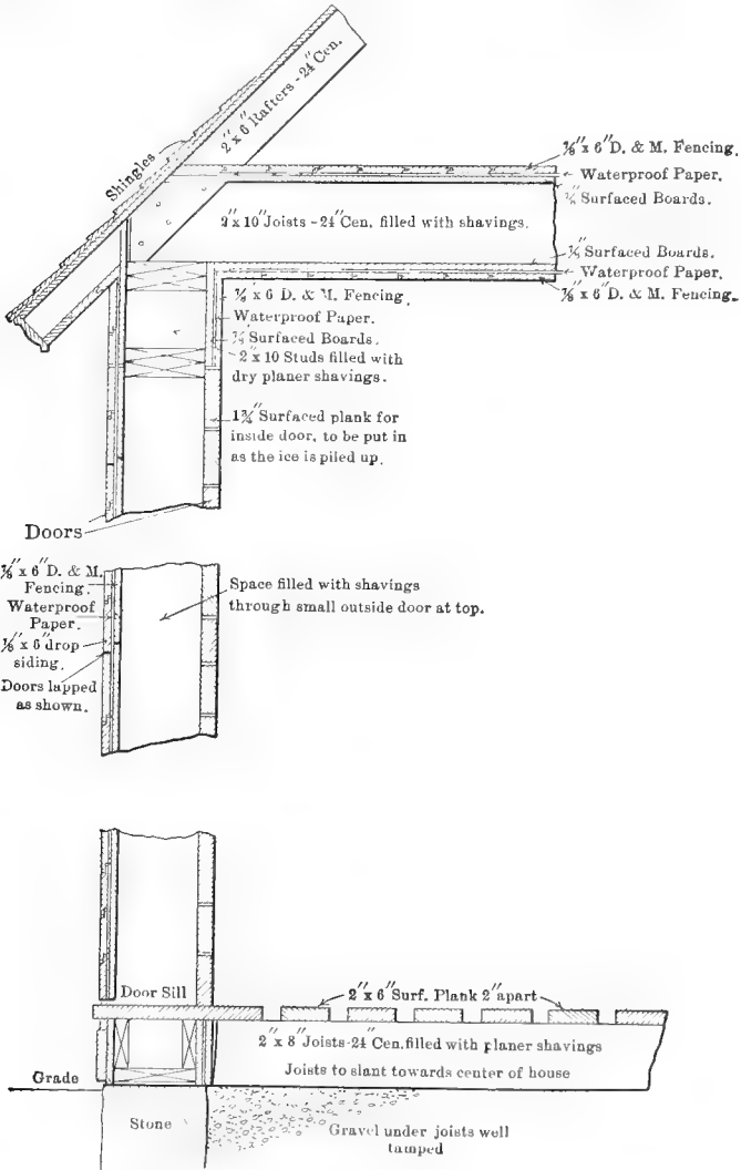
FIG. 131.—Construction detail of ice-house.
