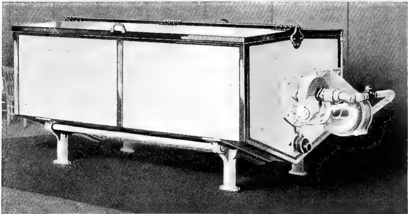
FIG. 71 — Progress vat pasteurizer and cream-ripener. (Davis-Watkins Dairymens Mfg. Co.)
