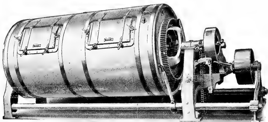
FIG. 90.—Master dual churn (Creamery Package Mfg. Co.)
