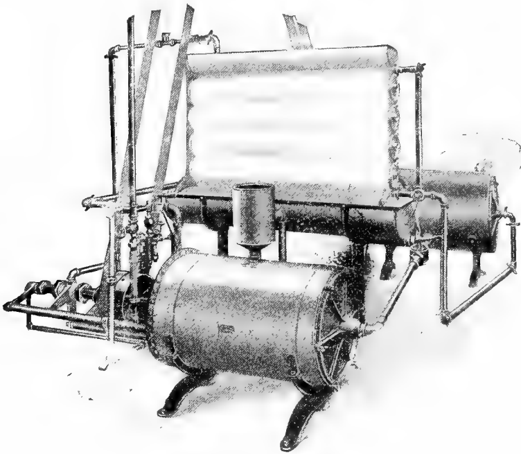
FIG. 69 -- Jensen sanitary pasteurizer-regenerator and cooler (Jensen Creamery Machinery Co.).
