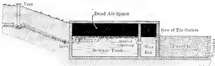
FIG. 122.—Cross-section of a sewage-disposal tank (Wallace's Farmer.)
