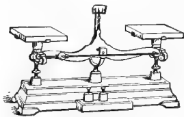
FIG. 19.—Troemner's Babcock cream-testing scales.
