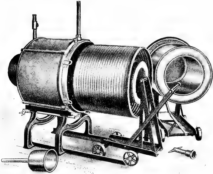
FIG. 66.—The Simplex regenerative pasteurizer (apart).
