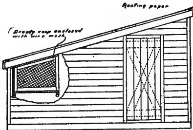
Side Elevation
