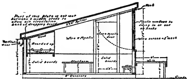
Cross Section
