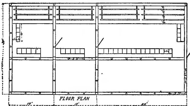
Details of the Clark semi-monitor, open-front house at the New Jersey State Experiment Station. A photograph of this house is shown on page facing 36
