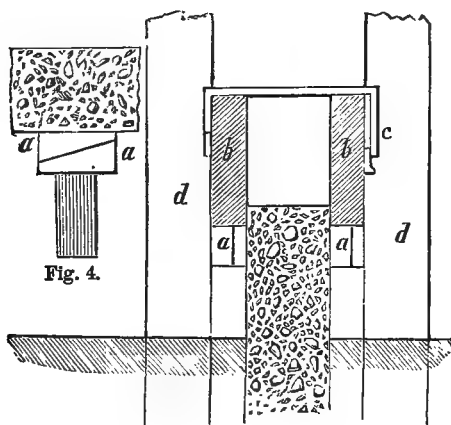
Figs. 4 and 5.—RAISING THE PLANKS.
