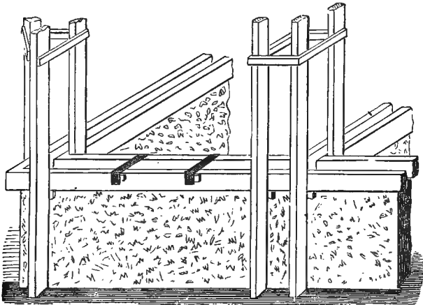
Fig. 3.—METHOD OF LAYING THE CONCRETE.
