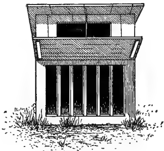
FIG. 62—SHADE BOARD
