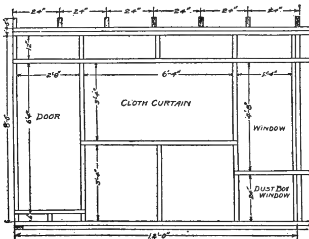
FIG. 9—FRONT ELEVATION OF FRAMEWORK
