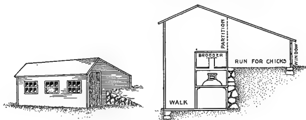
FIG. 75—SIDEHILL BROODER HOUSE
