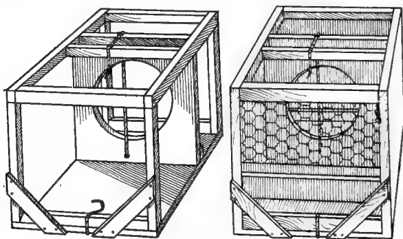
FIG. 27—MAINE TRAP NESTS
