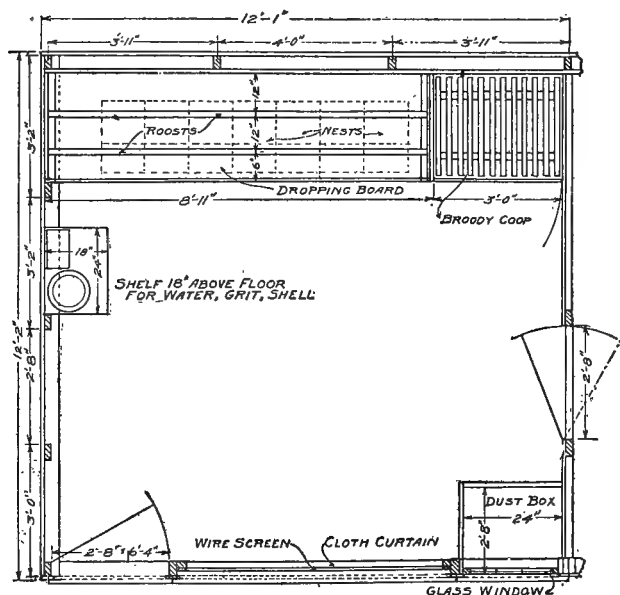
FIG. 10—GROUND PLAN CORNELL HOUSE
