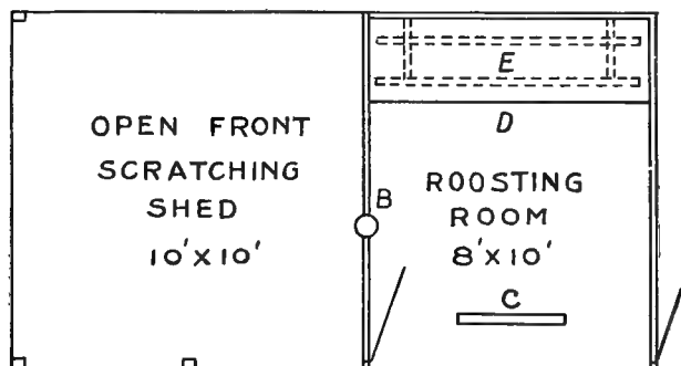
FIG. 3—GROUND PLAN OF SCRATCHING SHED HOUSE
