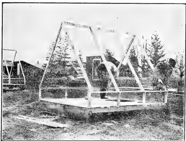
FIG 84—FRAME OF CORNELL COLONY-BROODER HOUSE
