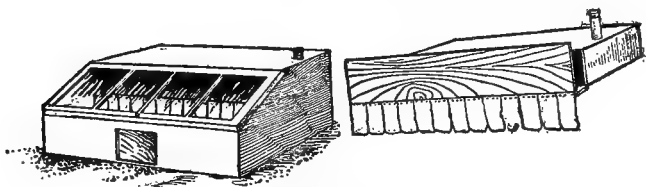
FIG. 89—HOT WATER BROODER AND TANK
