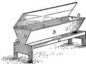
FIG. 47—SELF FEEDER
