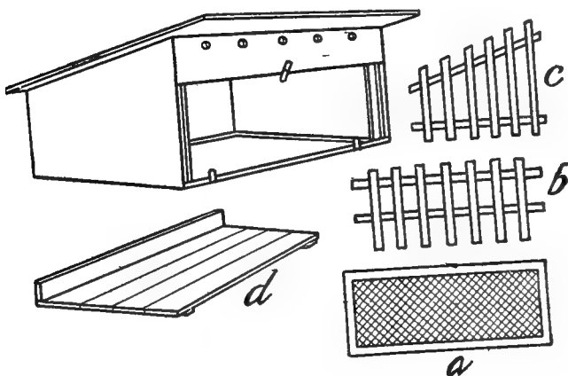
FIG. 63—COOP FOR TWO BROODS
