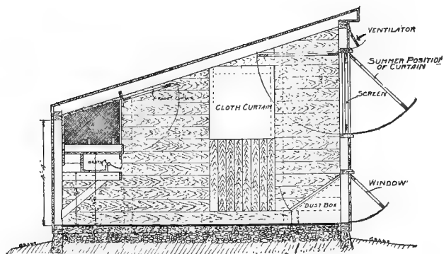
FIG. 8—SIDE VIEW CORNELL HOUSE
