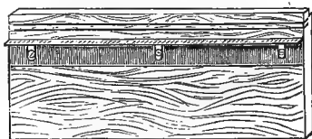
Side Wall of shallow extracting chamber, showing grooves for key and manner of raising frames, by adjusting the \frac{3}{8} -inch ledge upon which they rest. Keys can be dispensed with for old style of working.
