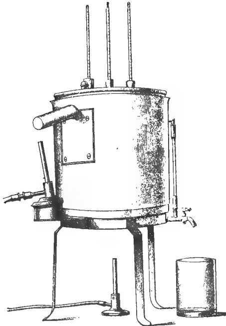
FIG. 52.—“Slow steriliser” for sterilising blood serum by Tyndall’s method, as adopted by Koch. For description see Fig. 53.
