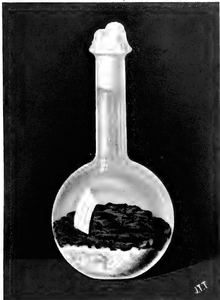
FIG. 28.— Aspergillus nigrescens growing on bread paste.
