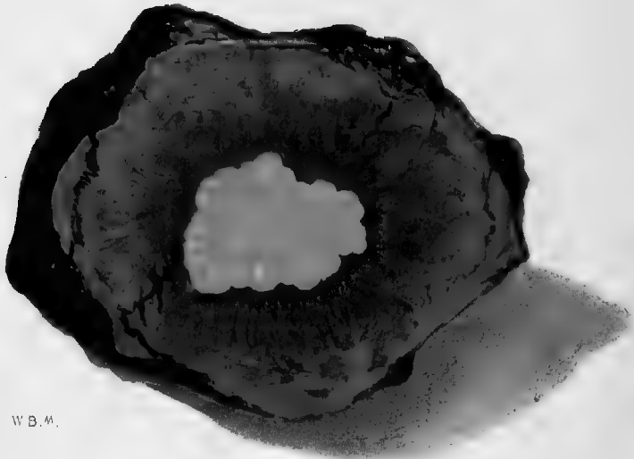
FIG. 15.— Bacillus anthracis growing on sterilised potato. The growth has a succulent appearance, and forms an elevated plateau with rounded edges.
