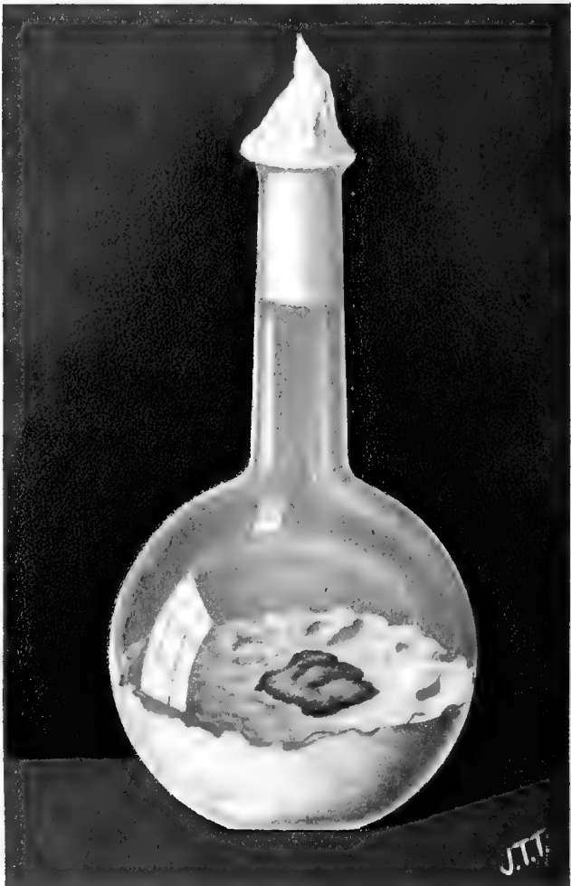
FIG. 25.— Aspergillus repens growing on bread paste—commencing growth. great importance, for upon their effectiveness as filters depends the purity of artificial cultures, not only in this special mode of cultivation, but in several of those to be mentioned subsequently.
