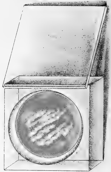
FIG. 56.—Tubercle bacillus upon solid serum.
