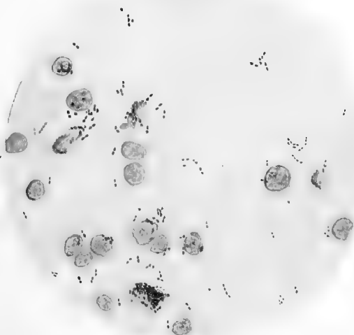
FIG. 3.--Blood taken from a case of traumatic tetanus. Blood corpuscles and micro-organisms stained with methyl violet, mounted in Canada balsam. ( \times 700 .)
