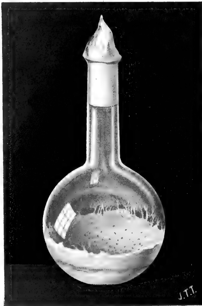
FIG. 23.— Mucor Lichtheimii growing on bread paste. On the surface of the delicate growth, small translucent yellow beads of liquid (which give an alkaline reaction) are seen.
