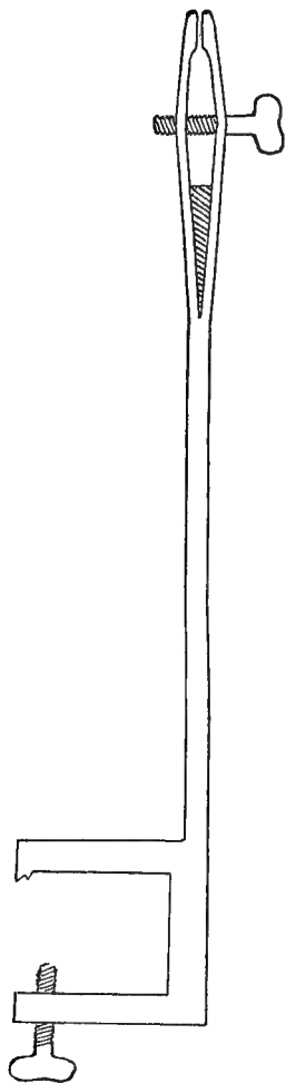
Fig. 54. — Fly-tyers' Vice.
