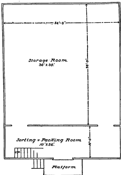
FIG. 56—PLAN OF STORAGE HOUSE
