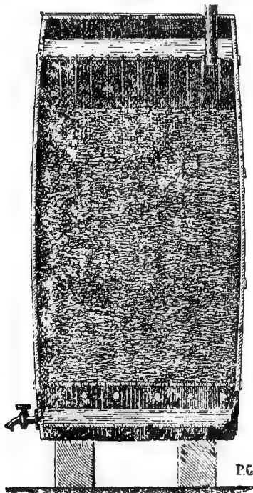
Vinegar generator (German method).
