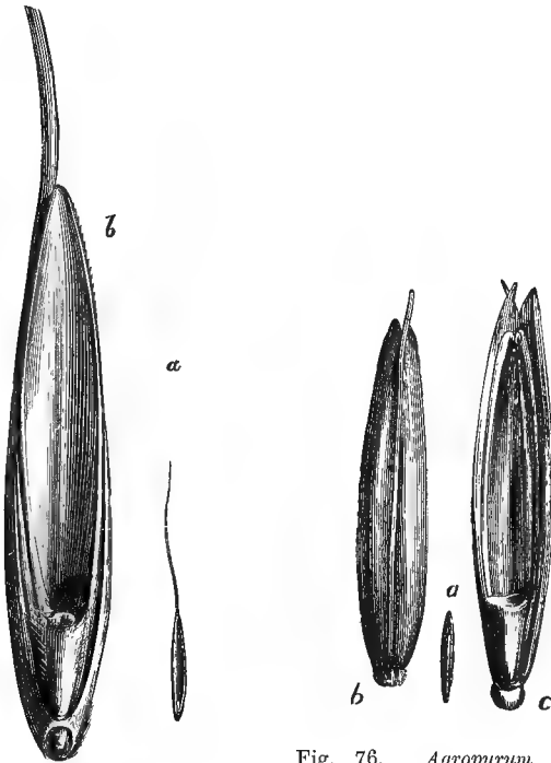
Fig. 75. Agropyrum caninum . Type of boat-shaped "seed" with sub-terminal awn. a , nat. size; b , \times about 9, but with awn cut short. Rachilla thicker above and hairy; palea not toothed. Nobbe. Cf. Fig. 48.
