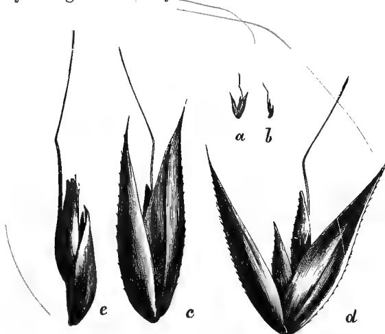
Fig. 66. Holcus mollis . Type of "double seed," which really consists of the entire spikelet ( a , nat. size; c and d , \times 8 ) comprised of the two glumes enclosing two pairs of paleæ and their enclosures ( b , nat. size; e , \times about 8). The lower pair of paleæ are devoid of awns and enclose the caryopsis: the upper pair have stamens only, and the outer palea has a dorsal kneed awn, not twisted or hooked. Nobbe.
