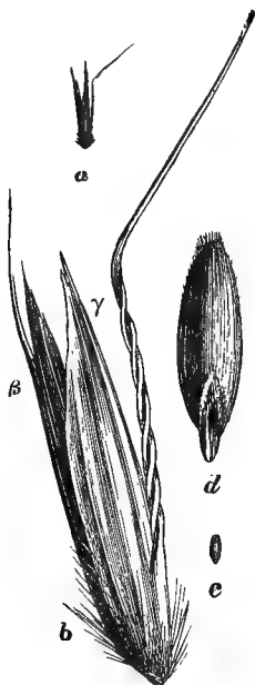
Fig. 47. Arrhenatherum avenaceum . The "double seed" (a and b) consists of two pairs of paleae with their enclosures. The lower pair ( \gamma ) are devoid of fruit, and the outer palea has a long twisted and kneed basal awn: the upper pair ( \beta ) enclose the fruit, and the palea has a short straight awn. Note the stiff basal hairs. a, nat. size; b, \times about 6; c, caryopsis, nat. size; d, ditto, \times 6. Nobbe.
