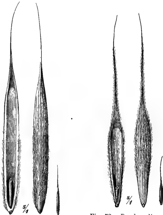
Fig. 72. Brachypodium sylvaticum , a barge-shaped "seed" with terminal awn, natural size and \times about 5. Cf. Fig. 77. Stebler.
