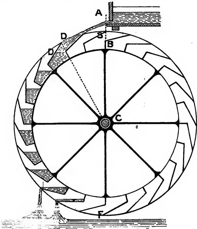
FIG. 12.—Overshot water wheel.
