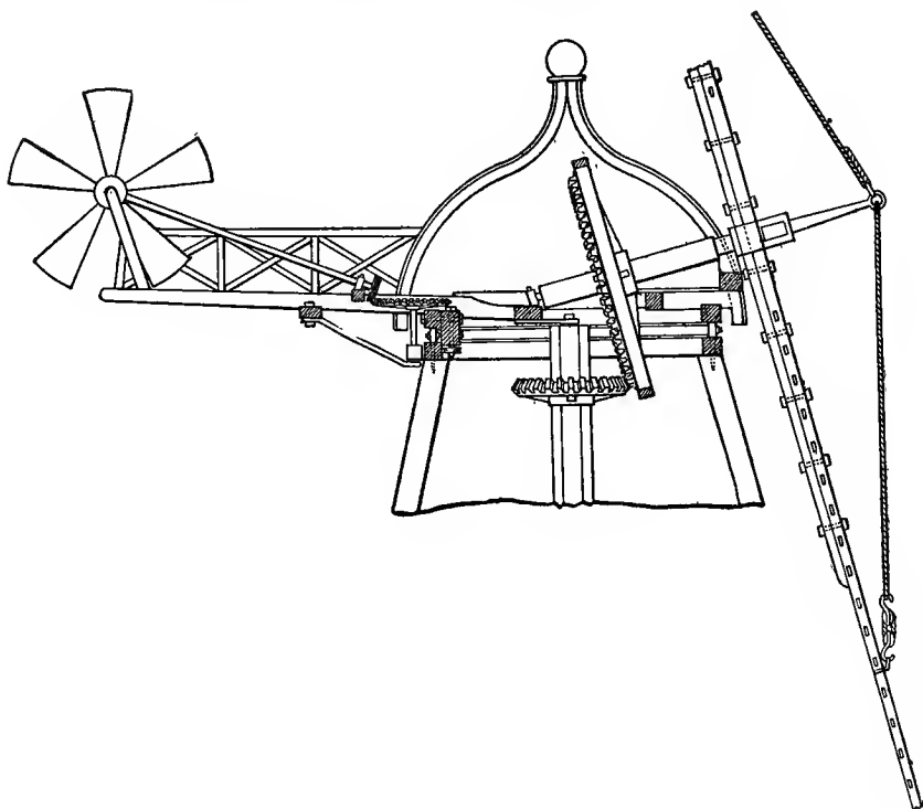
10.—Early form of head of tower windmill.
