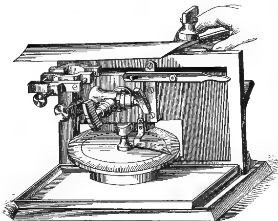
Schanze's microtome.
