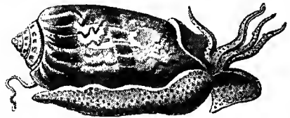
Fig. 184.—Olive ( Oliva )
