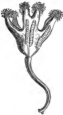
Fig. 296.— Lucernaria , enlarged
