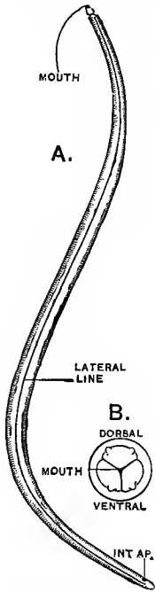
Fig. 276.—Round-Worm ( Ascaris )
