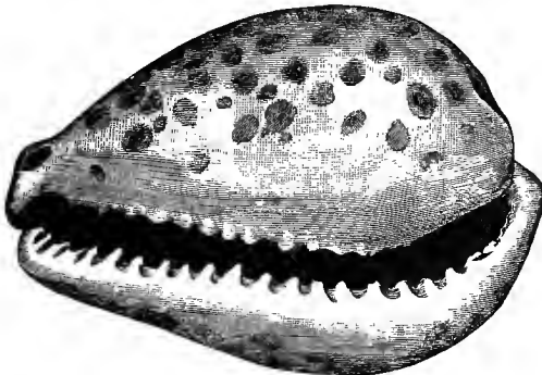
Fig. 186.— Cowry (Cypraea)
