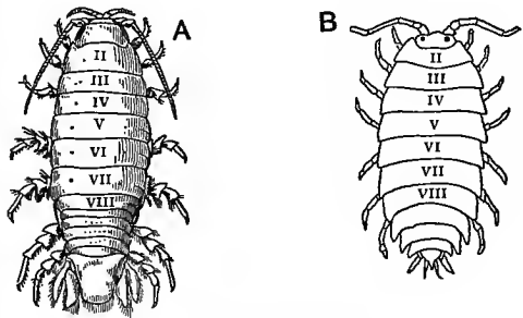
Fig. 256.—Isopods (enlarged)
