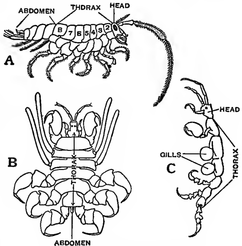
Fig. 255.—Amphipods (enlarged)
