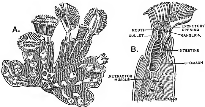
Fig. 270.—Polyzoa, enlarged
