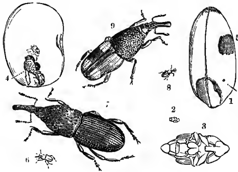
Fig. 222.—Corn-Weevil
