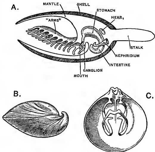
Fig. 271.—Lamp-Shell ( Waldheimia )
