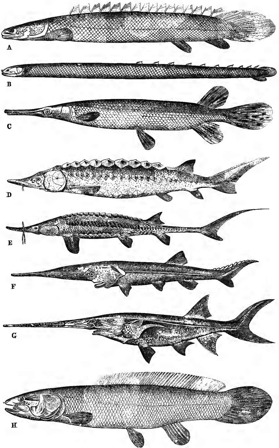
Fig. 162. —Ganoids
