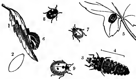
Fig. 216.—Lady-Birds
