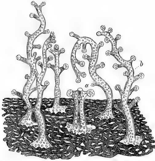
Fig. 2.—Enlarged view of a portion of the surface of a living colony of Millepora nodosa , showing the expanded zoöids of a single system. a , Central "gastrozooid;" b , One of the mouthless "dactylozoöids." (After Moseley.)
