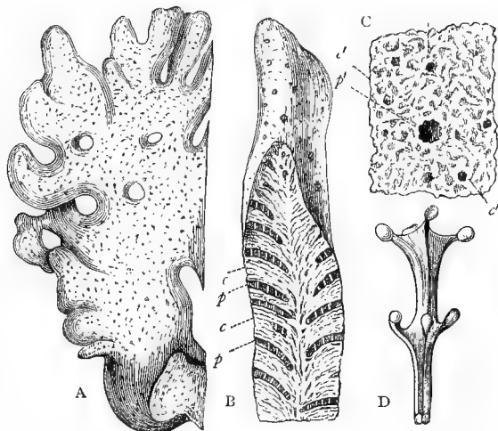
Fig. 1.—A, Portion of a mass of Millepora alcornis , of the natural size; B, Portion of the same, cut open vertically to show the larger tabulate tubes ( p, p ), and the spongy coenosarc skeleton ( c, c ), enlarged; C, Small portion of the surface, enlarged to show the larger and smaller openings ( p, c ) inhabited by the different zoöids, and the reticulated calcareous tissue of the skeleton; D, Part of a polypite, enlarged, showing two whorls of knobbed tentacles. (A, B, and C are after Milne-Edwards and Haime; D is after Martin Duncan and Major-General Nelson.)
