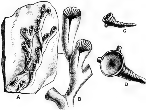
Fig. 8.—A, Portion of the corallum of Aulopora tubæformis , Goldf., from the Devonian of the Eifel, of the natural size; B, Two corallites of the same enlarged, showing septal striæ; C, Cladochonus ( Pyrgia ) Michelini , E. and H., Carboniferous, of the natural size; D, The same slightly enlarged, showing the interior of the calice.
