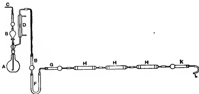
FIG. 5. — KNORR'S APPARATUS.
