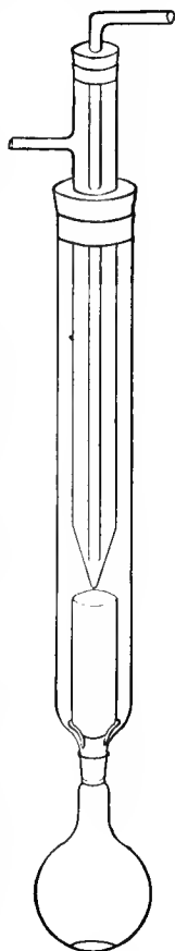
FIG. 2. EXTRACTION APPARATUS.
