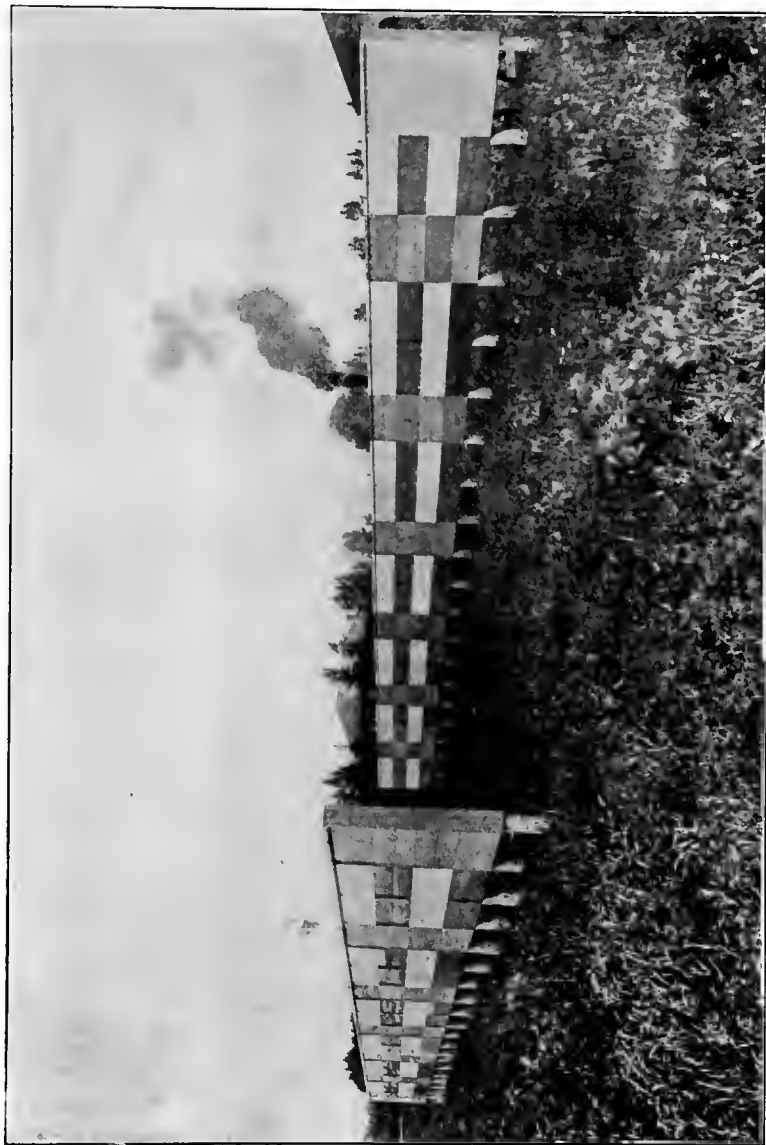
FIG. 7.—EXPOSURE FENCES, 1907.
