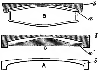
FIG. 190.—Methods of re-setting pieces split from the outline of the fiddle.
