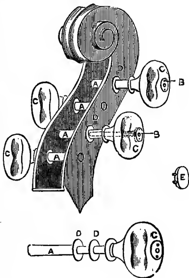
FIG. 97.—Wallis's Patent Peg.
