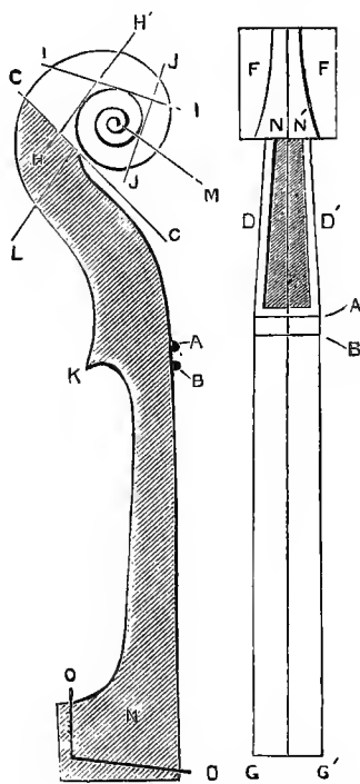
FIG. 164. — Commencement of cutting out Neck and Scroll.
