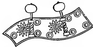
FIG. 96.—Machine-Head for Violin.
