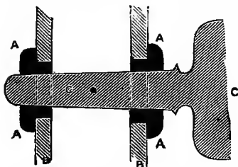
FIG. 98.—Patent Peg to ensure Firmness.
