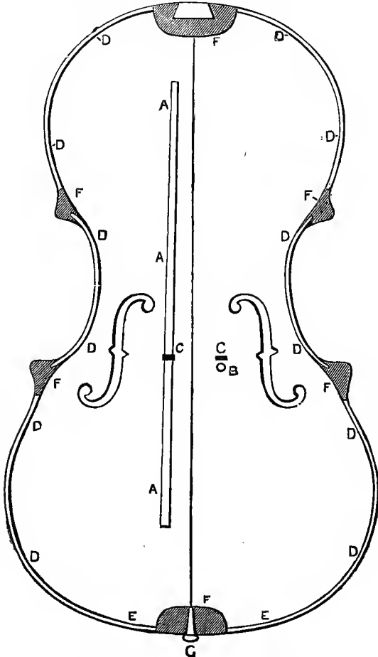
FIG. 82.—The Interior of the Violin.
