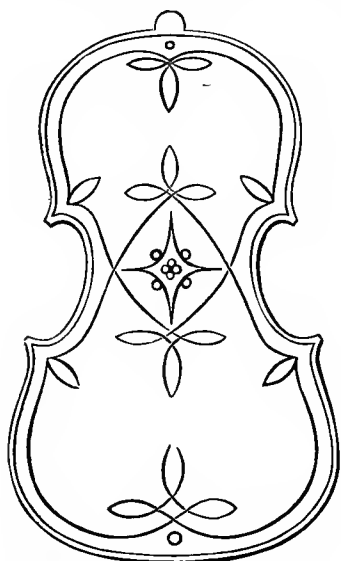
FIG. 91.—Ornamentally inlaid Purfling.
