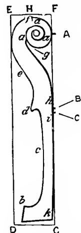
FIG. 161.—Plank outline of Neck and Scroll (on block).
