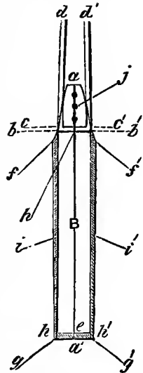
FIG. 196.—Operation of splicing head on to neck.
