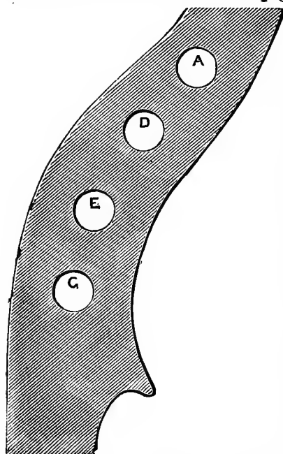
FIG. 187.—Setting of the pegs in the cheeks of the scroll.
