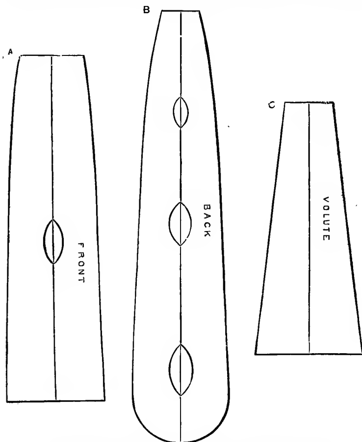
FIG. 162.—Outlines (Zinc) for marking front and back of Scroll (actual size).
