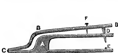
FIG. 128.—Gauging Callipers.
