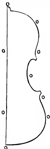
FIG. 173.—Half outline of Tables (back and belly).
