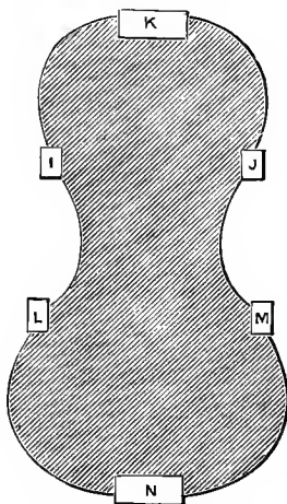
FIG. 175.—Inside mould, with rough blocks fitted.
