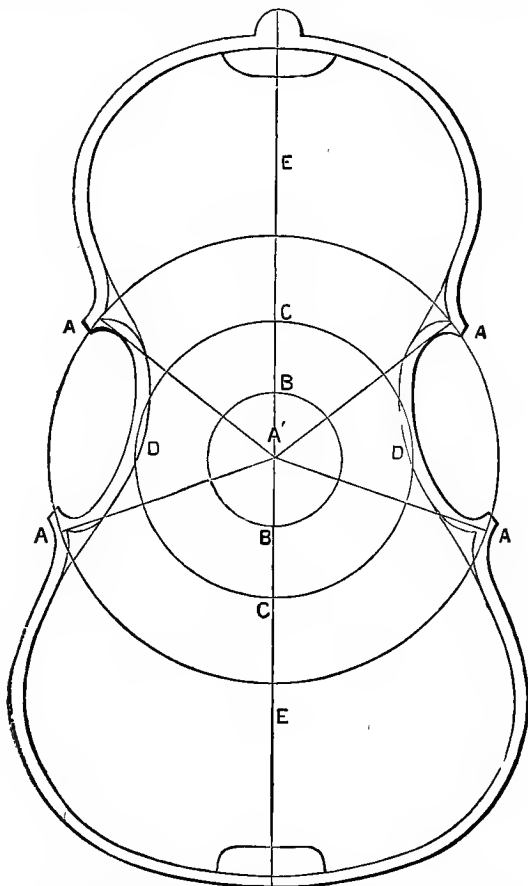
FIG. 149.—Diagram for regulating the thicknesses of the back.
