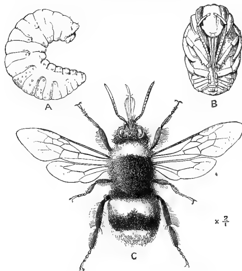
FIG. 331.— Bombus lucorum . A, Adult larva; B, pupa; C, imago, female. Britain.
