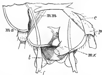
FIG. 242.—Transverse horizontal section of head of Psocus : f , fork or pick; t , lingua; mx , left maxilla; c , cardo; p , stipes; m.m. , muscles; m.s. , socket of mandible.
