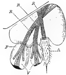
Fig. 95.—Abdominal appendage and exsertile vesicles of Machilis . A, appendage; V, vesicles protruded; P, basal portion; R, muscles. \times 70 .
