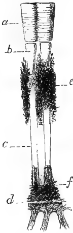
FIG. 53.—Two ommatidia from the eye of Colymbetes fuscus , \times 160 . (After Exner.) a , Cornea; b , crystalline cone; c , rhabdom; d , fenestrate membrane with nerve structures below it; e , iris-pigment; f , retina-pigment.
