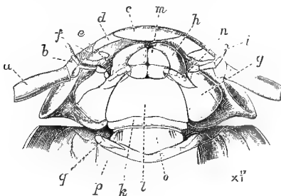
FIG. 115.—Under side of head and front of prothorax of Hemimerus . a , base of antenna; b , articulation of antenna; c , labrum; d , mandible; e , condyle of mandible; f , articular membrane of mandible; g , stipes of maxilla; h , exterior lobe; i , palpus of maxilla; k , submentum; l , mentum; m , terminal lobe of labium; n , labial palp; o , plate between submentum and sternum; p , prosternum; q , cervical sclerites. (After Hansen.)
