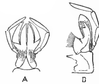
FIG. 226. — Termes bellicosus . Labium, A, maxilla, B, of winged adult; lower face of each. (After Hagen.)
