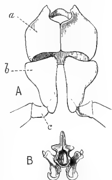
FIG. 335.—Articulation of front legs of the hornet ( Vespa crabro , ♀). A : a , side-piece of prothorax overlying the prosternum; b , coxa; c , trochanter. B , prosternum proper, as seen from front when extracted.
