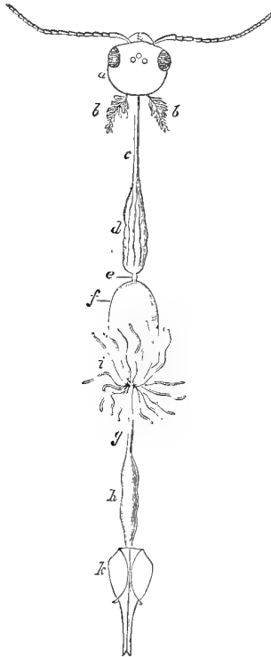
FIG. 69. — Digestive system of Xyphidria camelus (after Dufour): a , head capsule; b , salivary glands; c , oesophagus; d , crop; e , proventriculus; f , chyle, or true stomach; g , small intestine; h , large intestine; i , Malpighian tubes; k , termination of body.
