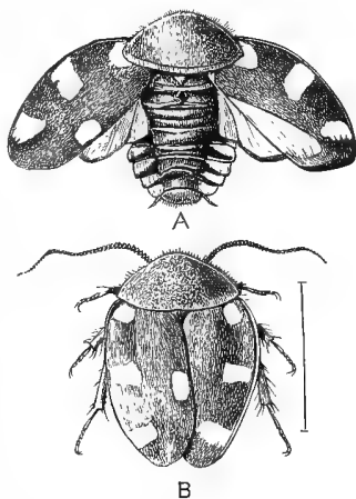
FIG. 128.— Corydia petiveriana , with tegmina extended, A; closed, B.
