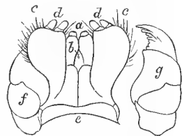
FIG. 33. — Mouth parts of Chilognatha . (From C. L. Koch, Die System der Myriapoden .) f and g , The mandibles. The parts marked a , b , c , d , e are firmly united and constitute the broad plate No. 3. They have received the following names— a , b , Internal stipes; c , external stipes; d , malellae; e , hypostoma.
