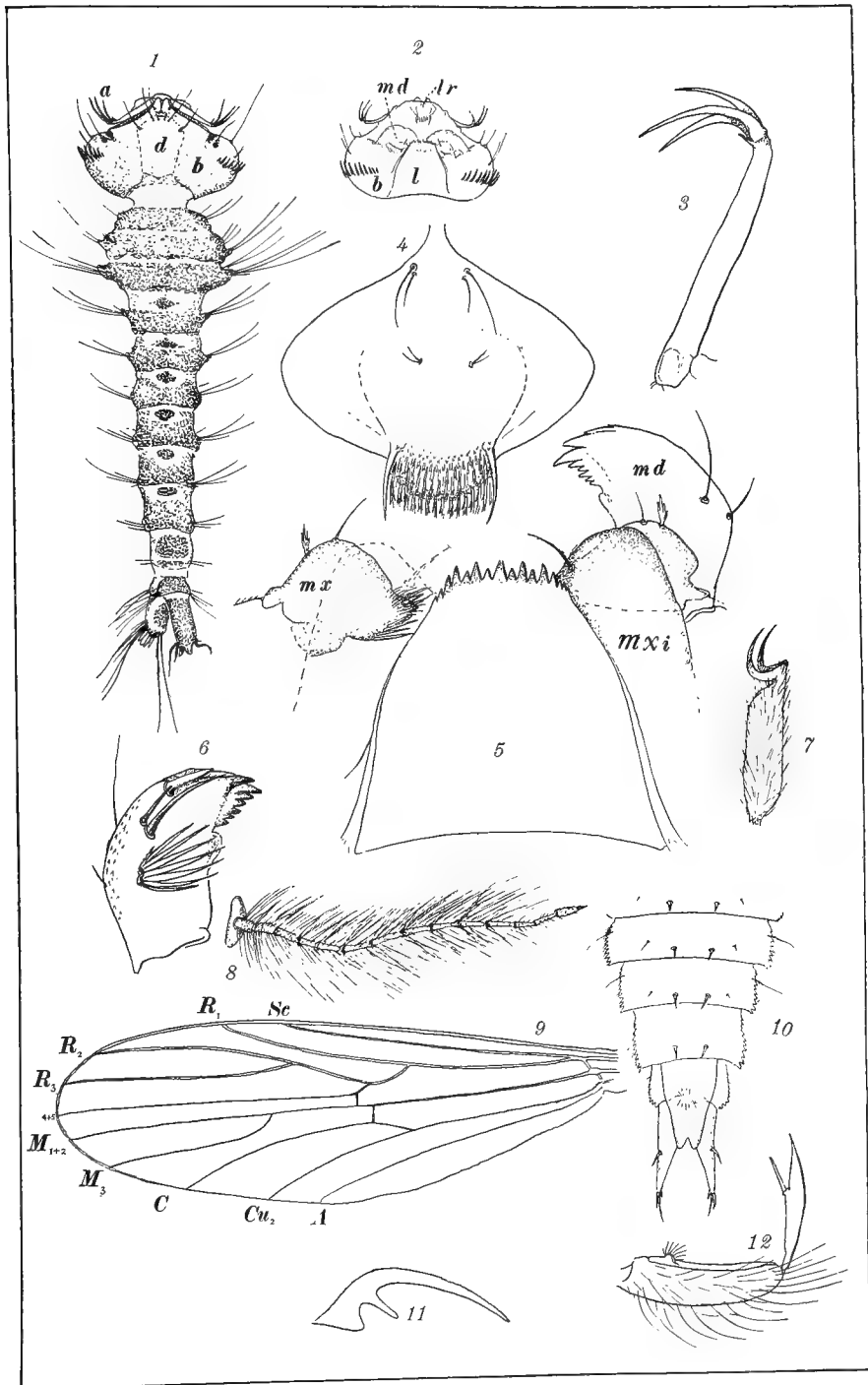
Ceratophrella brakeleyi
