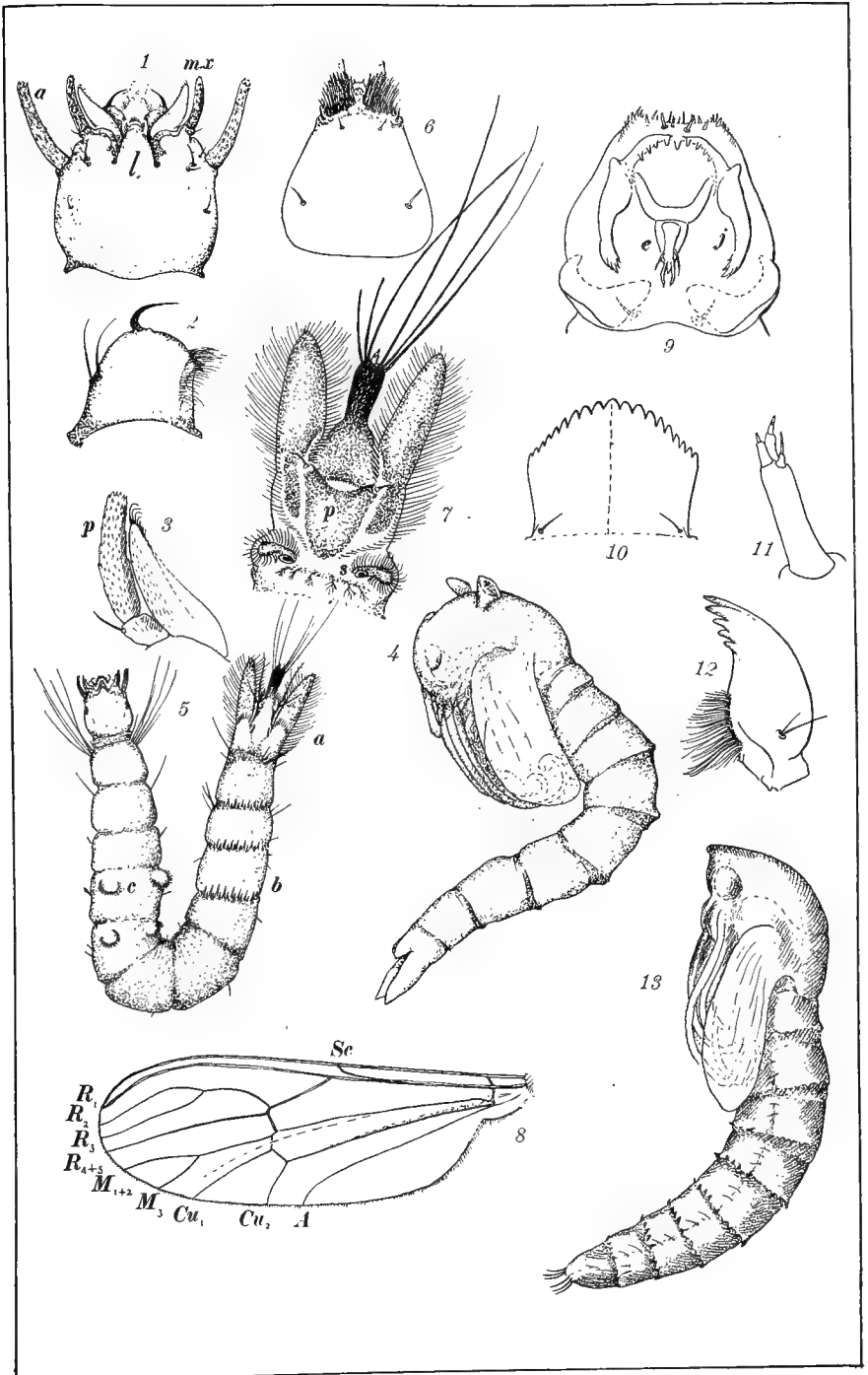
Diamesa waltlii
