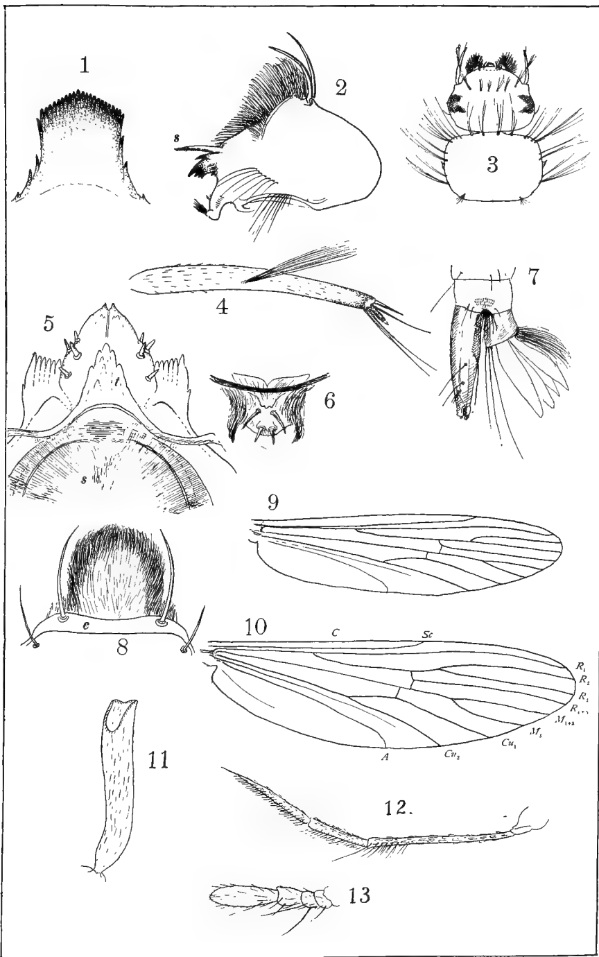
Gulex restuans
