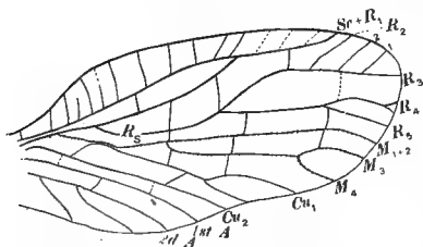
Fig. 23 Forewing of Sialis infumata x4
