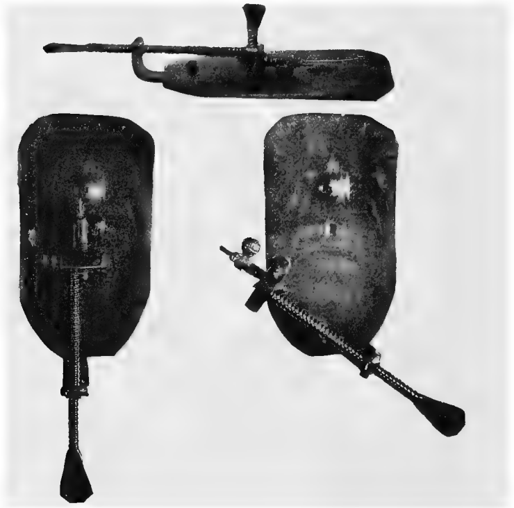
FIG. 19.—LEEUVENHOEK'S MICROSCOPE.
