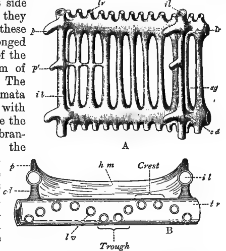
FIG. 6.—A. Part of branchial sac of Ascidia from inside. B. Transverse section of same. tv , transverse vessel; cd , connecting duct; hm , horizontal membrane; il , internal longitudinal bar; lv , fine longitudinal vessels; p , p' , papillæ; sg , stigmata. A and B are drawn to different scales. (From Herdman, Challenger Report.)
