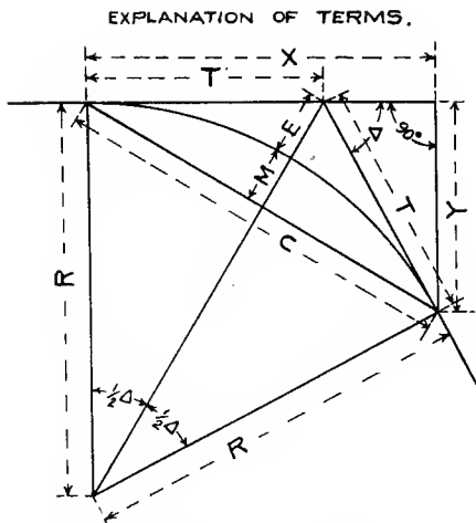
FORMULAS FOR A 1^\circ CURVE.
