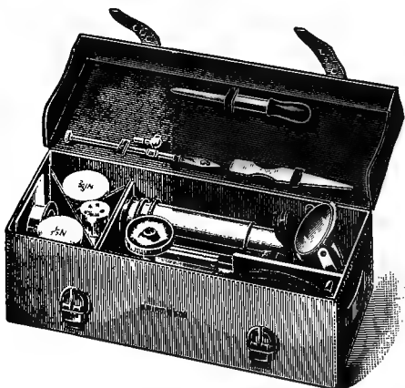
FIG. 4.—Portable Microscope.
