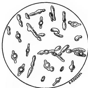
FIG. 21.—Spindle-shaped yeast.
