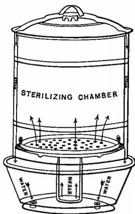
FIG. 81. Steam sterilizing apparatus.
