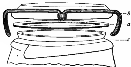
FIG. 65. The top of a common fruit jar; a is the rubber ring upon which the success of the sealing is dependent.
