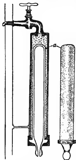
FIG. 76. Pasteur filter, showing the filter itself, a , made of unbaked porcelain, and the metal cover.
