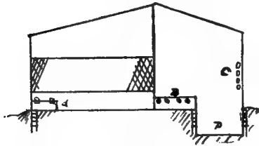
Fig. 31. Cross Section of Long Brooder House — pipe system — single row of pens.
