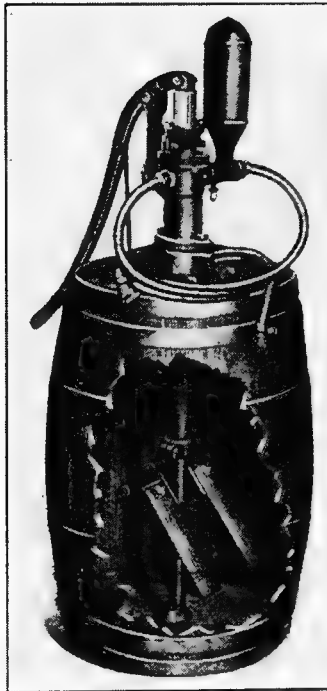
FIG. 239.—Spray barrel with pump.
