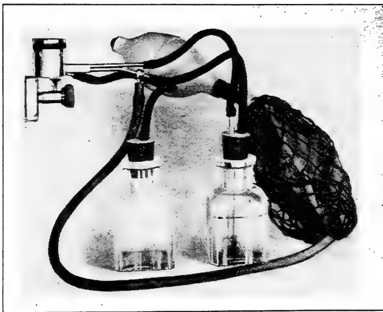
FIG. 233.—Ether or rhigoline freezing attachment for freezing microtomæ.
