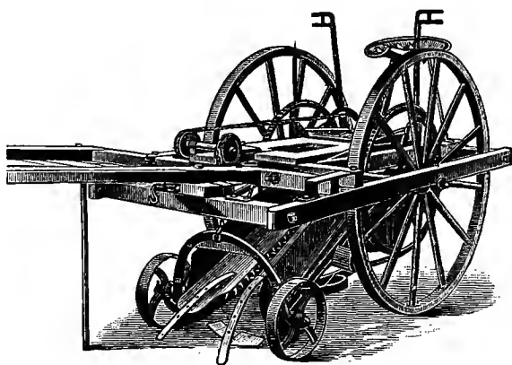
BEAN HARVESTER.
