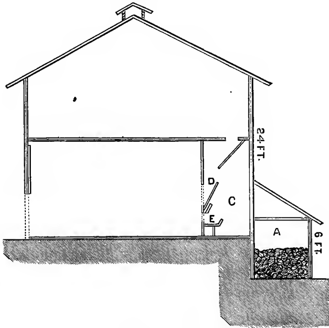
SECTIONAL VIEW OF SHEEP BARN.
