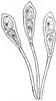
FIG. 141.—The winter spores of wheat-rust.
