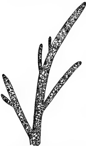
FIG. 98.— Cladophora : a branching filament, each of whose cells contains several nuclei.
