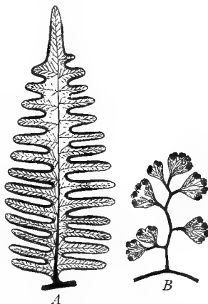
FIG. 183.—Sporangia of ferns, showing marginal lines of sporangia protected by the inrolled margin of the leaf: A, the common brake; B, maidenhair fern.
