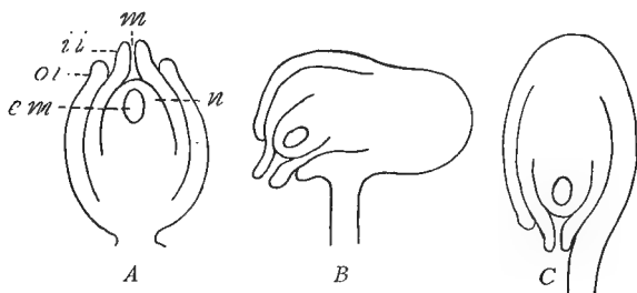
FIG. 217.—Diagrammatic longitudinal sections of ovules, showing outer ( oi ) and inner ( ii ) integuments, micropyle ( m ), nucellus ( n ), and megaspore ( em ), the last often called embryo sac: A , erect ovule; B , curved ovule; C , inverted ovule.
