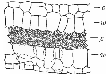
FIG. 24.—Section through a leaf of Be-sonia , showing epidermal layers ( e ), colorless water storage tissue ( w ), and the central cells containing chloroplasts ( c ).
