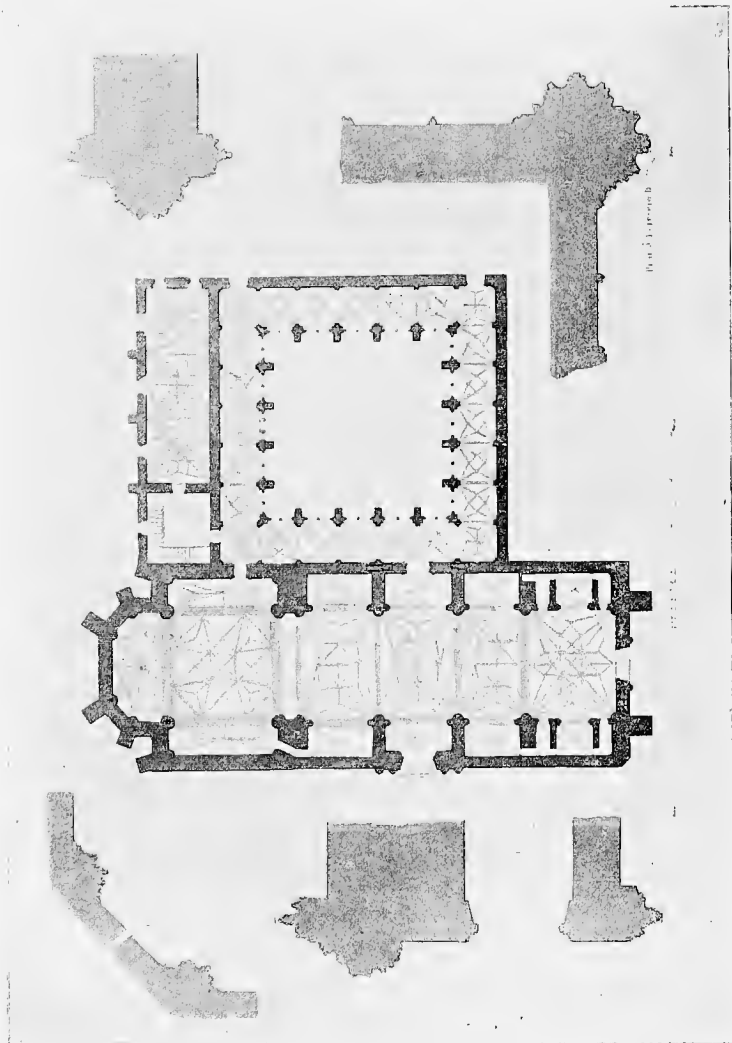
PLAN OF THE CHURCH AND PROFESSIONAL CLOISTER OF SAN JUAN DE LOS REYES
