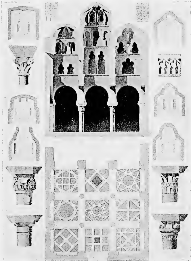
ANCIENT MOSQUE, NOW THE HERMITAGE OF SANTO CRISTO DE LA LUZ
