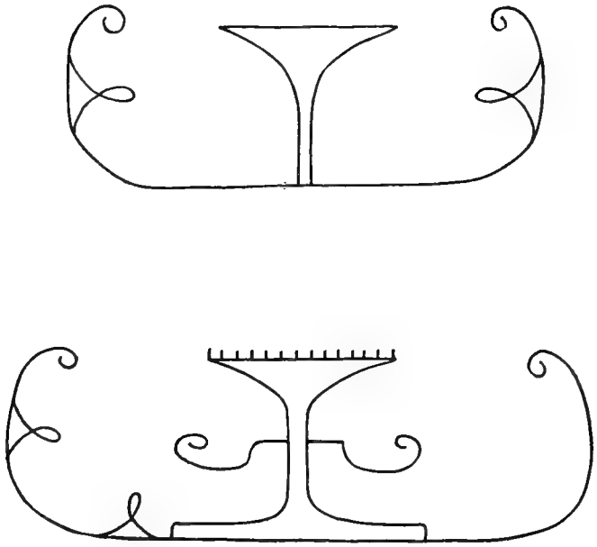
Fig. 9. Micmac double-curve designs.
