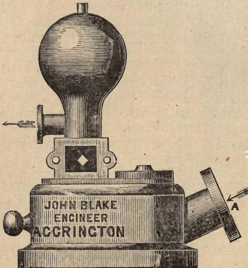
DIRECT ACTION RAM.
