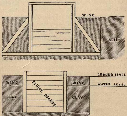
REARING STREAM SLUICES.
