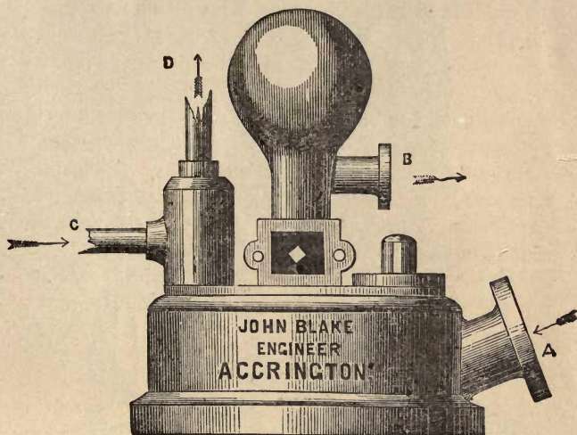
SECONDARY ACTION RAM.
