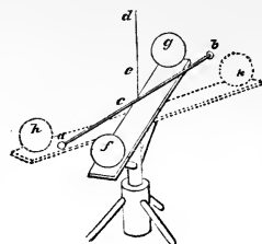
Michell's Torsion Balance.
