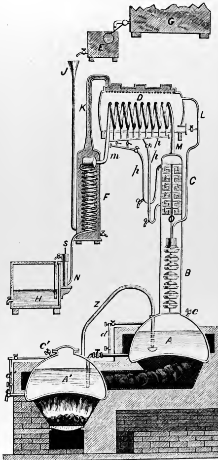
FIG. 4.—Derosne's Still.
