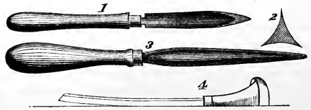
Fig. 3.—Steel Engraver's Tools. 1. Scraper. 2. End View of Scraper. 3. Burnisher. 4. Burin.
