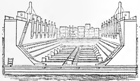
FIG. 5.—Balance Dock.
