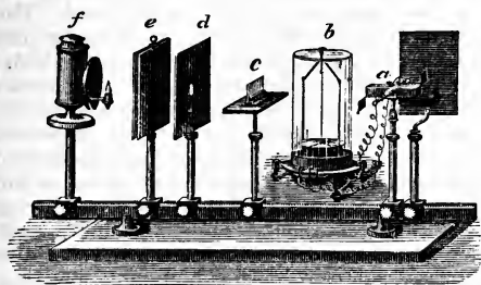
Melloni's Apparatus.
