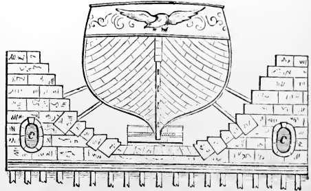
FIG. 4.—Transverse Section of Brooklyn Dry Dock.
