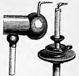
Fig. 13.—Current shown by means of a Flame.
