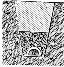
FIG. 1.—Section of an Underground Drain.
