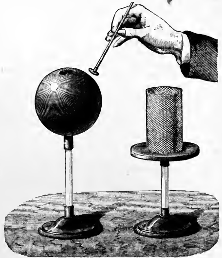
FIG. 5.—Proof Plane and Hollow Sphere.
