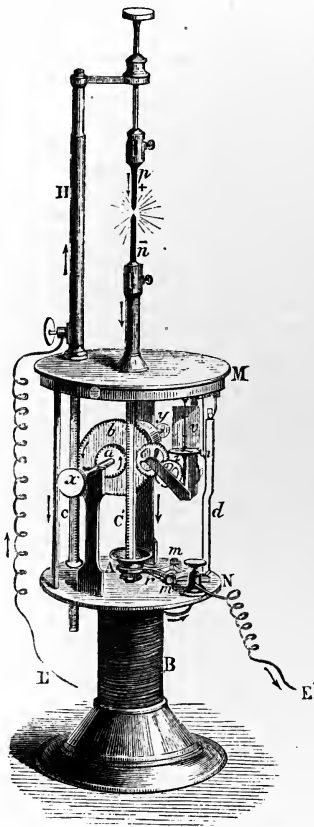
Duboscq's Regulator.
