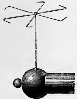
Fig. 12.—Revolving Points.
