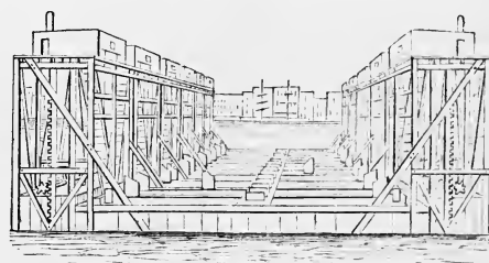
Fig. 7.—New York Sectional Dock.
