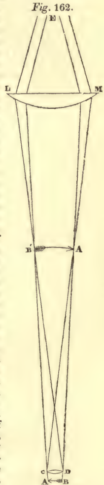
A B, the object, of which an amplified image is formed by the object-glass C D, in the contrary direction, at A' B', by the convergence of the rays of the several pencils to a focus. These again diverging are received by the eye-glass L M, which gives them the nearly parallel direction necessary for them to enter the eye, and causes the apparent size of the image to be E.
