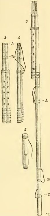
Modern Egyptian Pipes: Figs. 3, 4, the Zumnára (14 in. long); 5, mouth- piece of the latter; 6, the Argúhíl (3 ft. 2 in. long); each in sections, A-B, etc.
