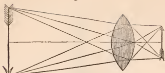
Formation of images by convex lenses.
