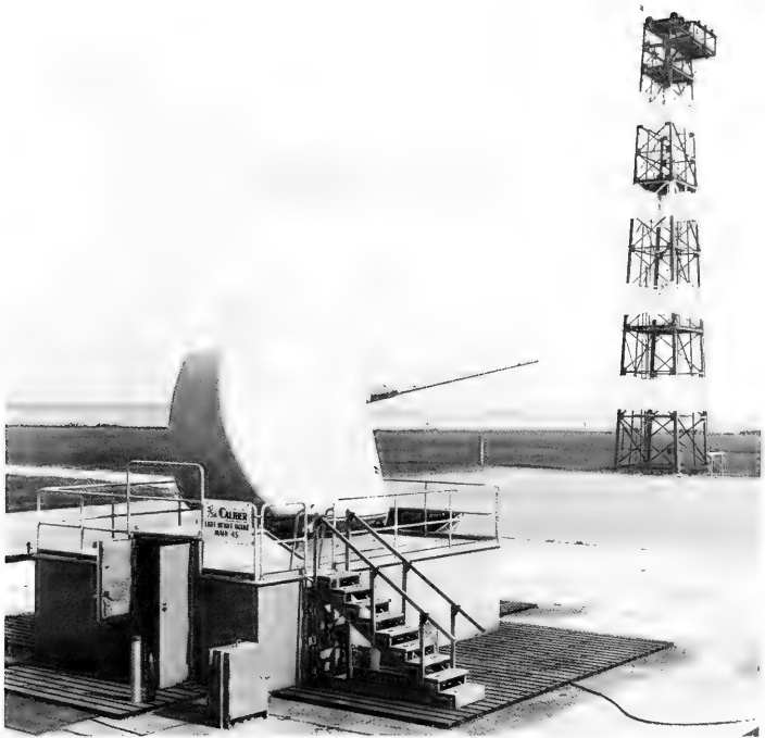
5"/54 MARK 45 installed for testing at Dahlgren.
