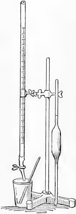
Apparatus for acid test.
