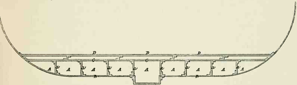
SECTION OF DOUBLE BOTTOM. From Patent Specification.
