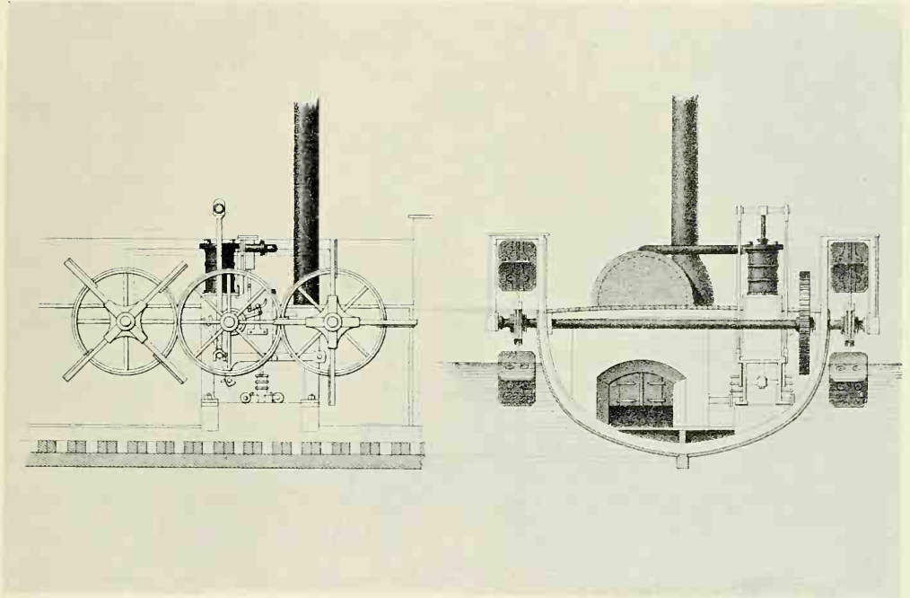
"COMET'S" ENGINES.
