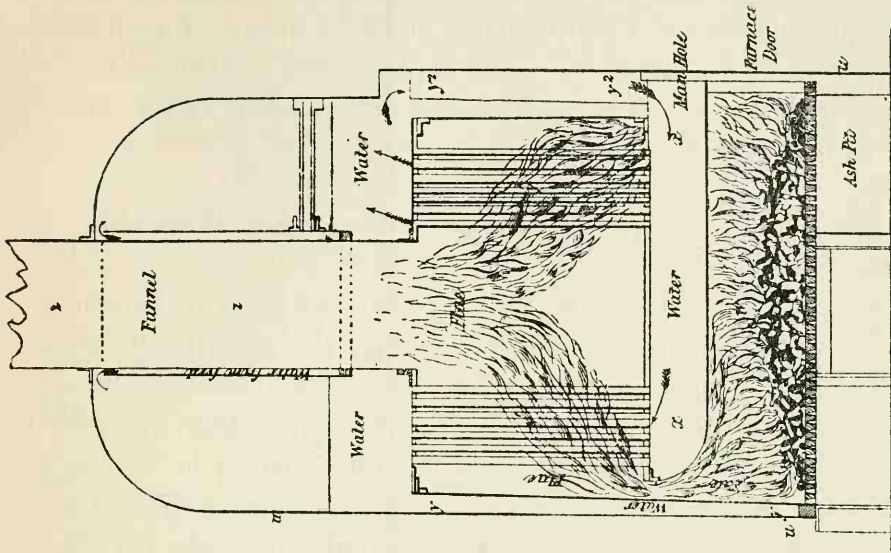
WATER TUBE BOILER, VERTICAL SECTION. From Patent Specification.
