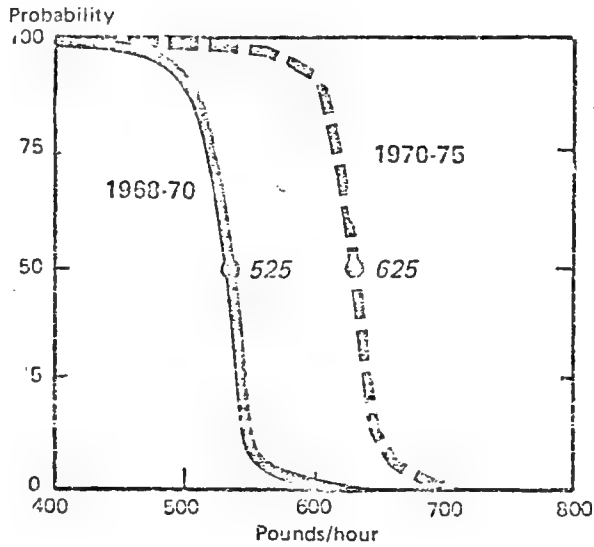
EXTRUDER RATE*
