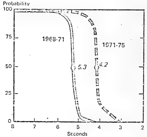
THERMOFORMER CYCLE TIME*
