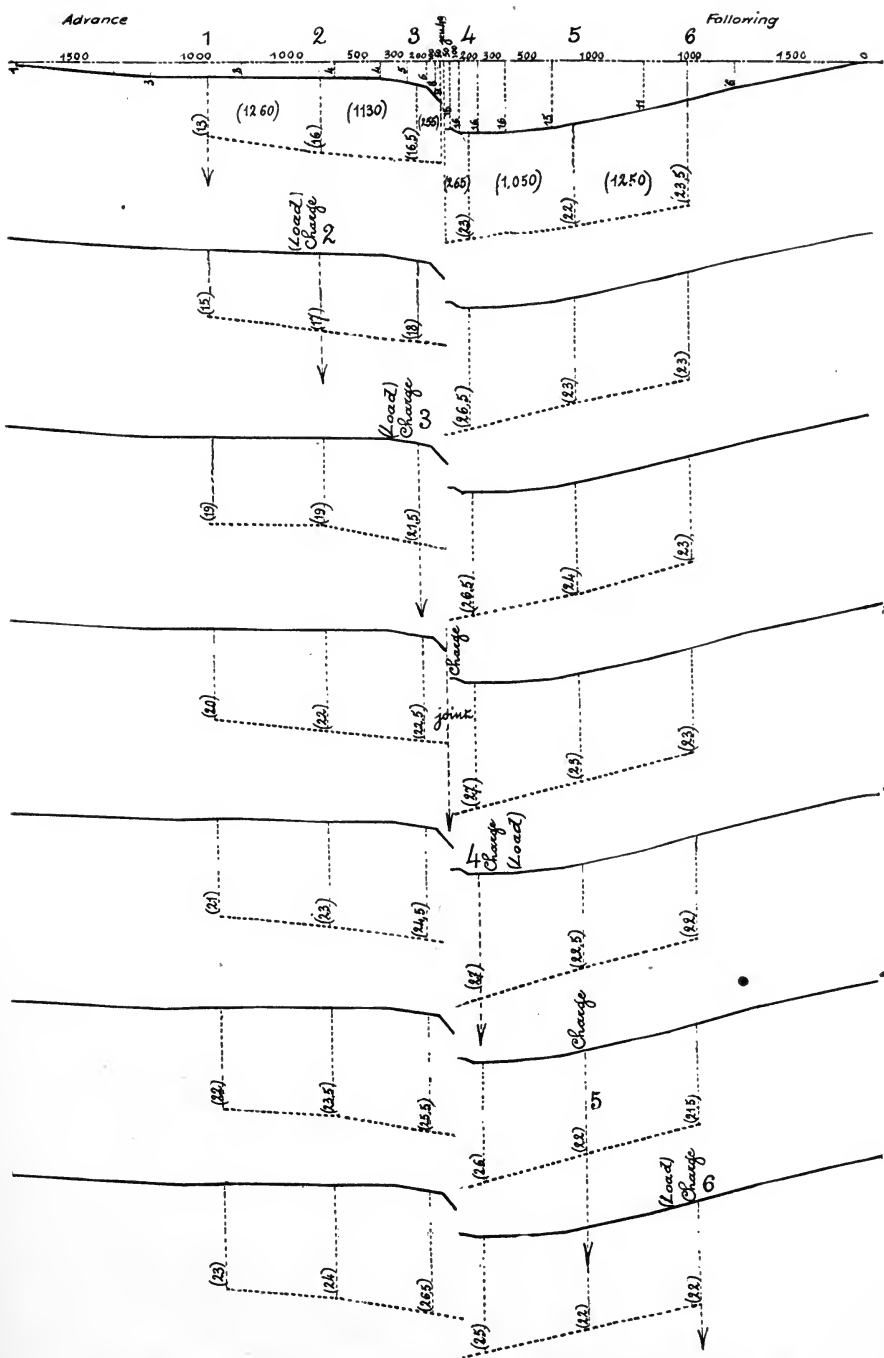
Fig. 22—Depression at the Joint at Passage of Train, Oak Ties.
