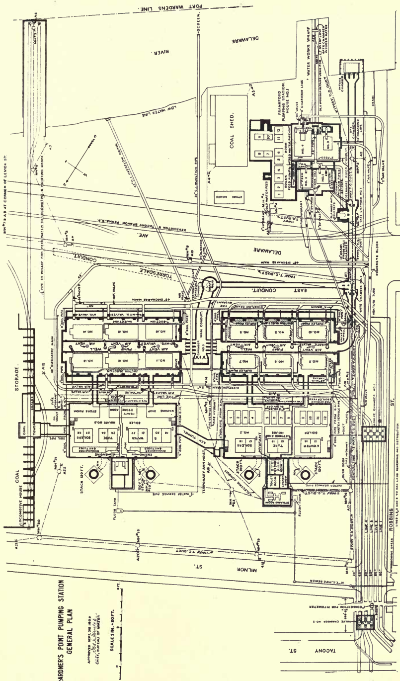
Lardner's Point Pumping Station. General Plan.
