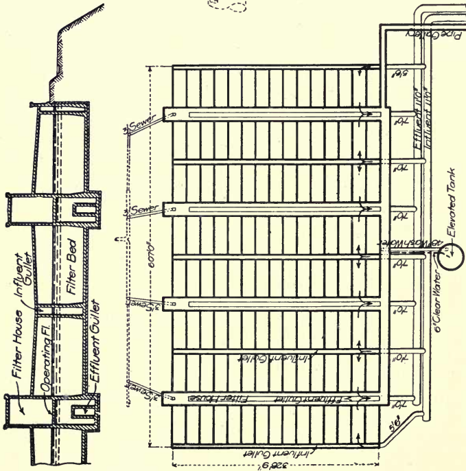
Part Sectional Plan of Plant.
