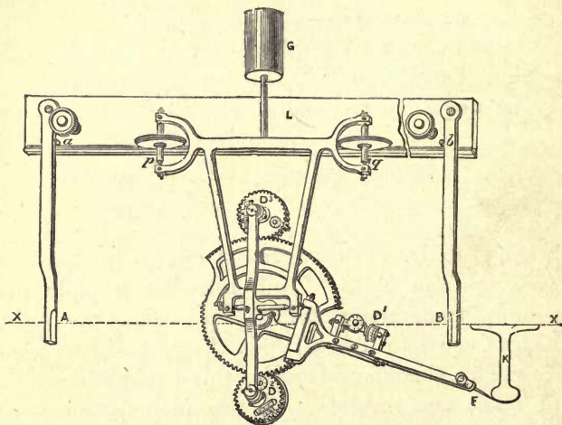
Amsler's Integrater.
