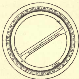
Inclination Protractor.
