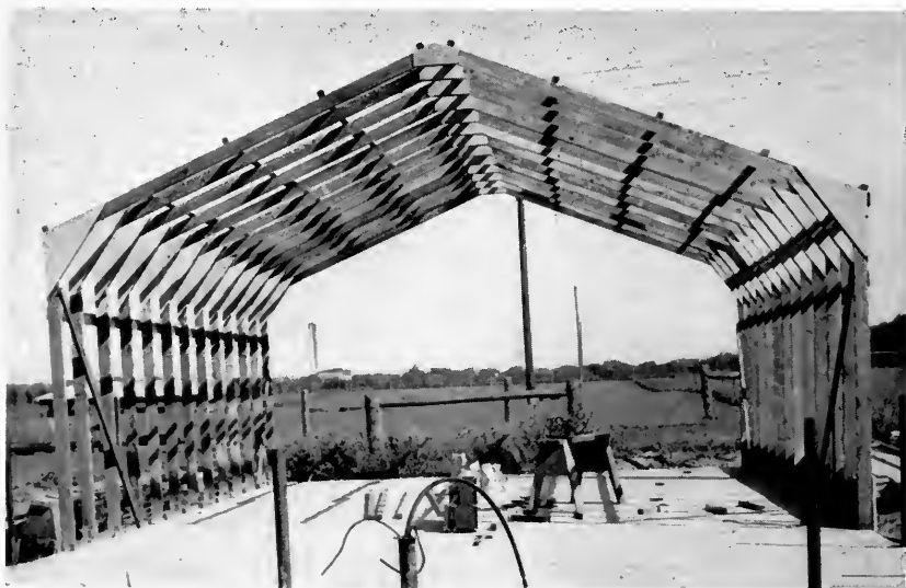
This framework of a small experimental swine shelter shows the type of rigid-frame design being developed. (Fig. 1)
