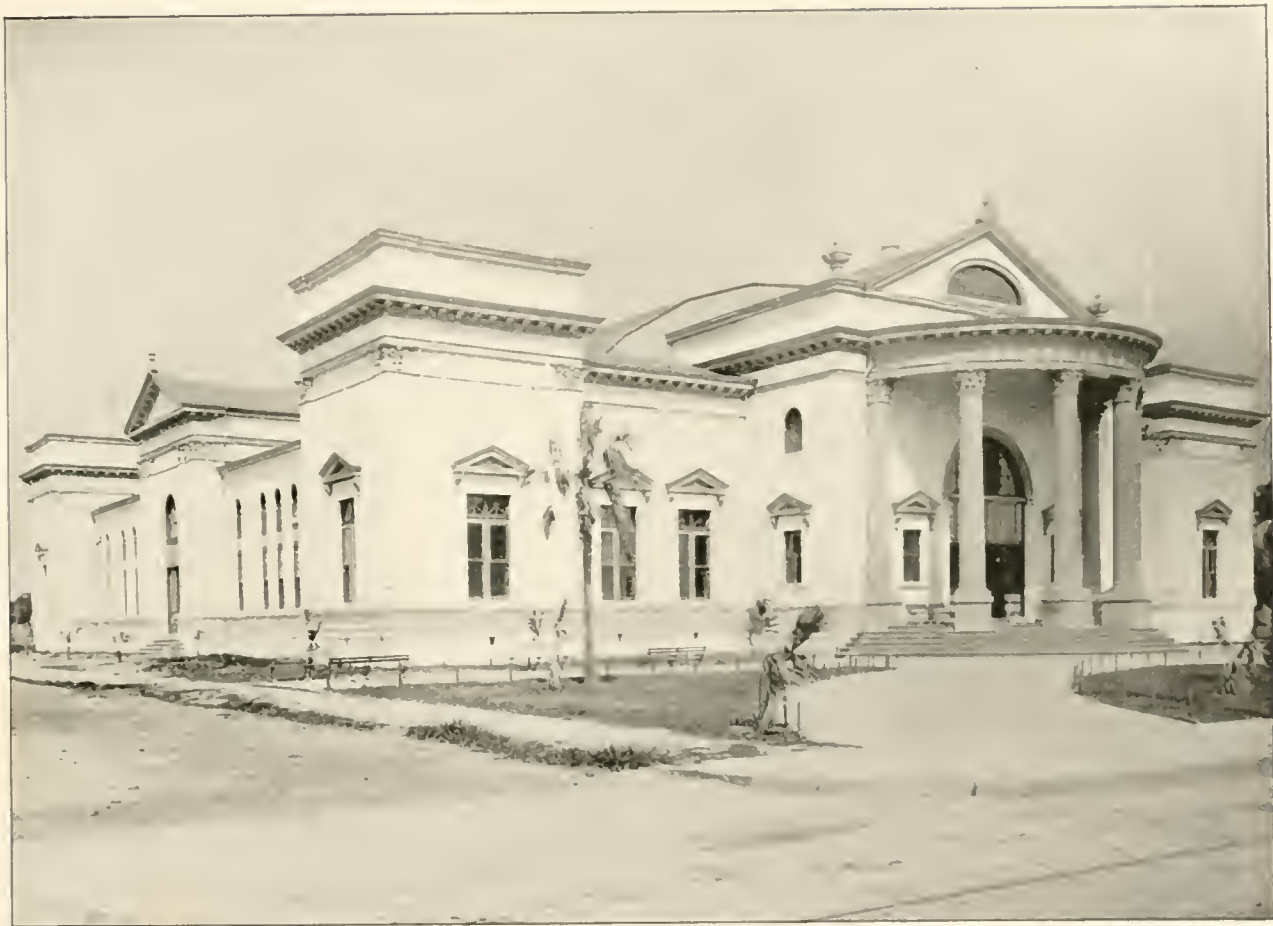
FRANK P. MILBURN, Architect. THOMSON AUDITORIUM. Charleston, S. C. Built by the city for the Confederate Veterans' Reunion, 1899. Erected in ninety days. Seating capacity 10,000; size 166x271 ft. McCarrell & Son, Builders.
