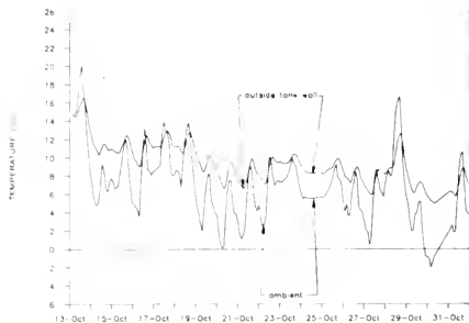
Figure 3.2 1983 autumn data at north side of an uninsulated tank (ROCKWOOD)
