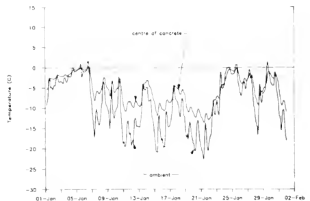
Figure 3.4 1984 winter data on north side of an uninsulated tank (ROCKWOOD)
