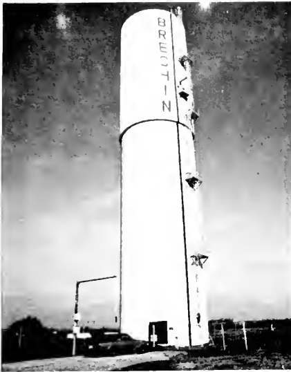
Photo 5-17 Tank after rehabilitation including strengthening by post-tensioning, installation of new steel liner, and insulation and cladding. (BRECHIN)
