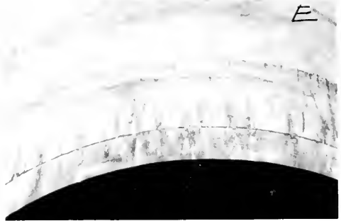
Photo 5-19 Vertical cracking at base of wall due to ineffective prestressing. This was caused by inadequate provision for inward movement between internal thrust ring and wall. (CHELMSFORD)
