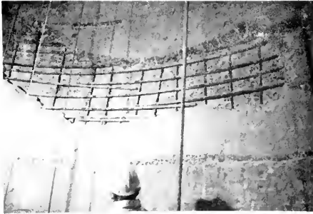
Photo 2-9 Internal delamination (ALVINSTON)
