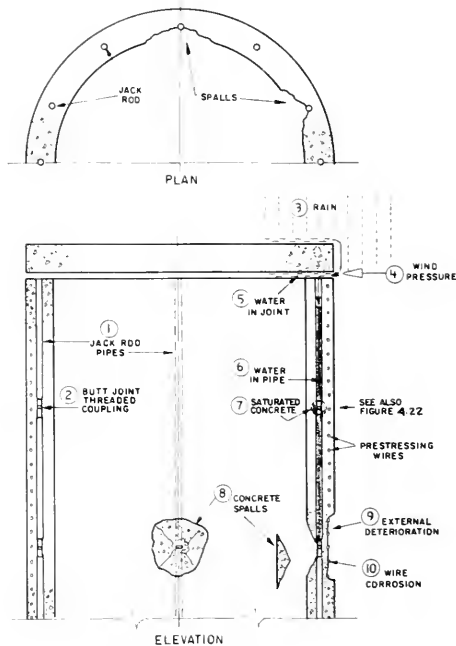
Figure 2.2 Jack-rod spalls
