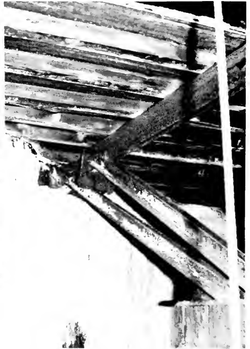
Photo 6-8 Corroded roof truss (HESPELER)
