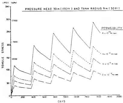
Figure 4.15 Permeability and tensile stress for 30m (100 ft.) head
