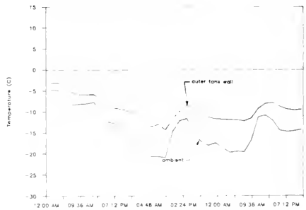
Figure 3.10 Daily temperature cycles showing continuous freezing at the North side of the tank
