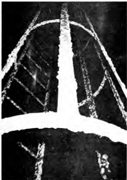
Photo 6-10 Aluminium ladder exhibiting severe pitting corrosion (BRIGDEN)
