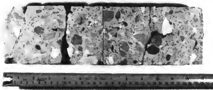
Photo 2-5 Core section showing fracture at external and internal steel (CAMLACHIE)
