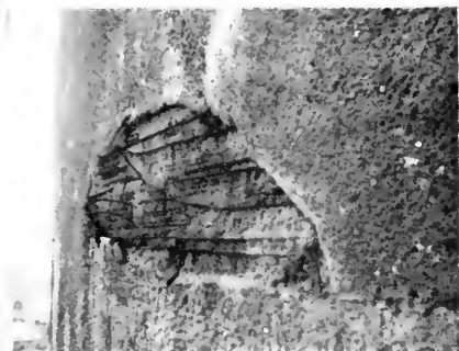
Photo 6-5 Delaminated cover coat exposing broken prestressing wires (AMHERSTBURG)
