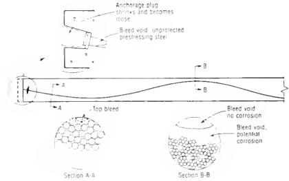
Figure 6.1 Bonded tendons. Bleed void, corrosion of unprotected prestressing steel. Concrete anchorage pocket plug shrinks (large circle, upper left) and becomes loose. Poor bond or non-expansive mortar permit aggressive materials access to anchorage and prestressing steel, likewise with improperly bonded and anchored exterior-end anchorage (shown at left end of prestressing steel) protection. (ref. 35)
