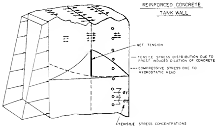
Figure 4.19 Distribution of stresses in tank wall section under increasing linear water pressure.
